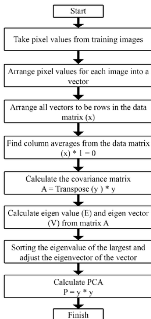
Fig. 1. Image Processing Phase with PCA
