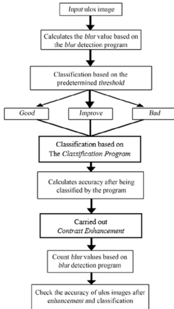
Fig. 3. Process Ulos image evaluation based on blur parameters
