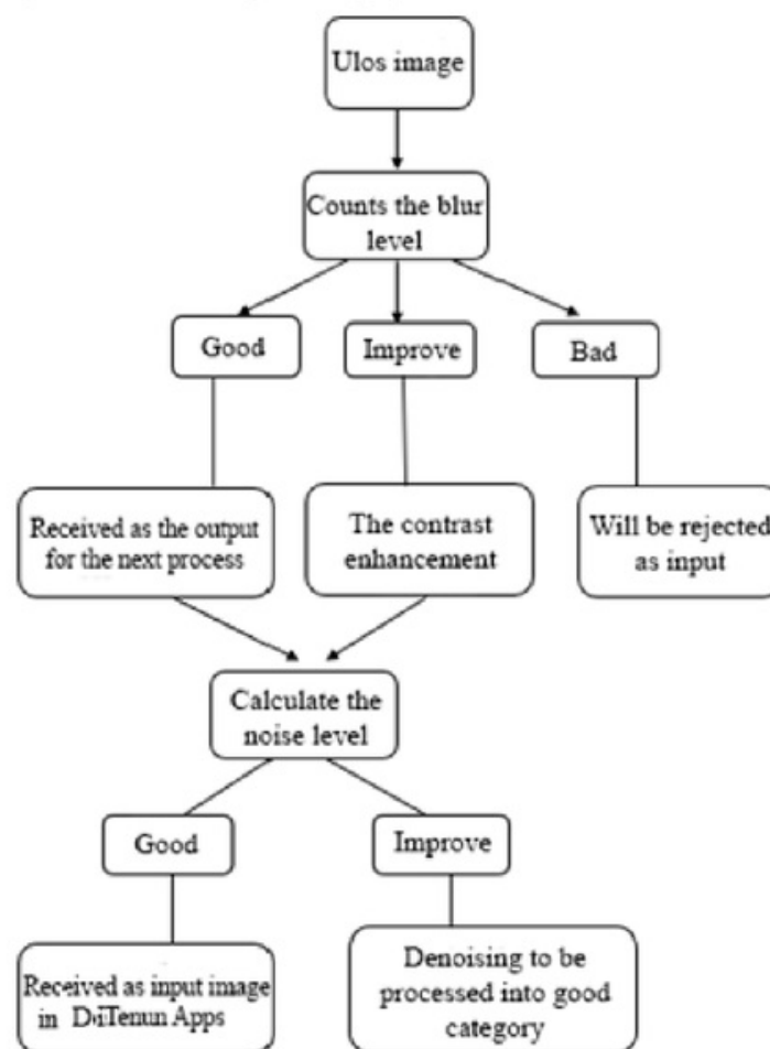
Fig. 5. Evaluation process Image blur and noise
