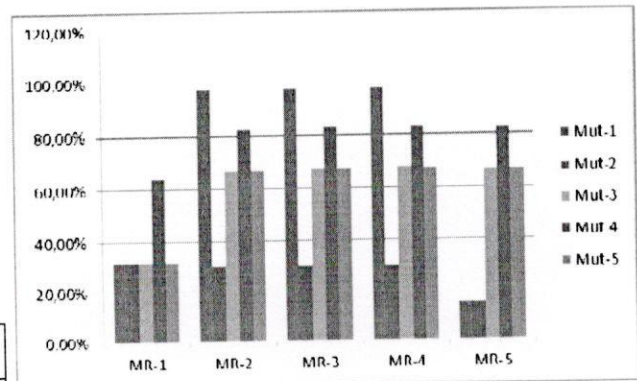
Figure-2. Average percentage number of pair test cases revealing errors.
